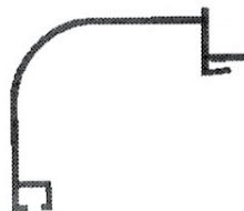
ALUMINIUM TOP POP-TOP EXTRUSION 6.5M LONG 007137
